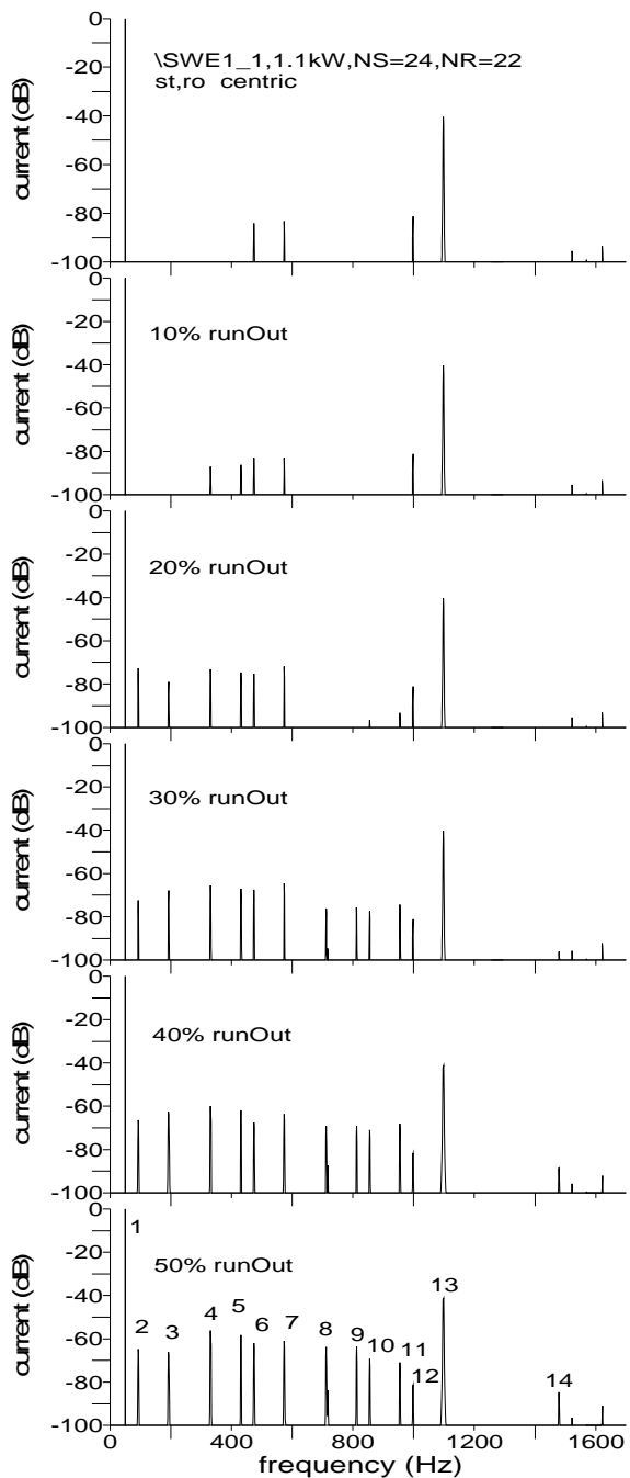
Fig. 1. Stator current harmonics (in decibels referred to a 50 Hz harmonic) for 8\text{-}\varphi vibrations of the rotor, for zero to 50% of the air gap length (thickness).
